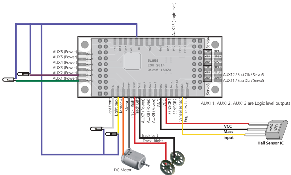
Figure 14: General Connection diagram LokPilot 5 L (Example wiring), Decoder plugged into the adapter board 51959
