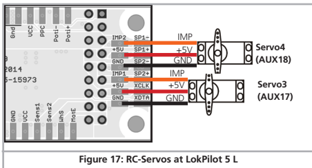
Figure 17: RC-Servos at LokPilot 5 L
